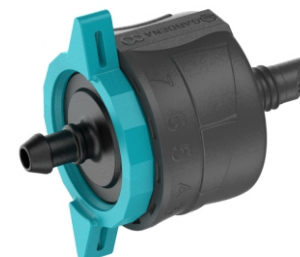
Micro-Drip-System Adjustable Endline Drip Head
